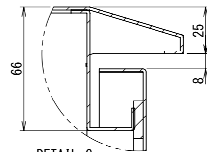
DETAIL G SCALE 1 : 2
