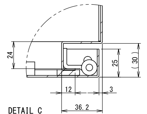
DETAIL C SCALE 1 : 2
