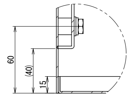
DETAIL F SCALE 1 : 2
