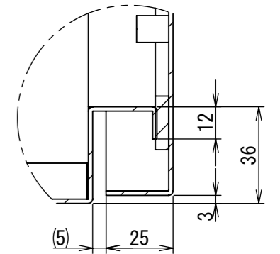
DETAIL E SCALE 1 : 2
