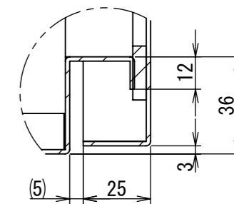
DETAIL E SCALE 1 : 2
