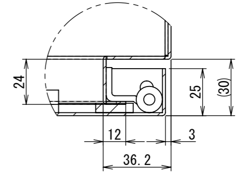
DETAIL AE SCALE 1 : 2
