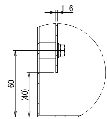
DETAIL F SCALE 1 : 2
