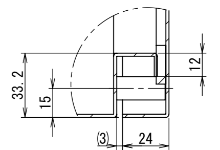
DETAIL E SCALE 1 : 2
