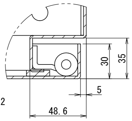
DETAIL R SCALE 1 : 2
