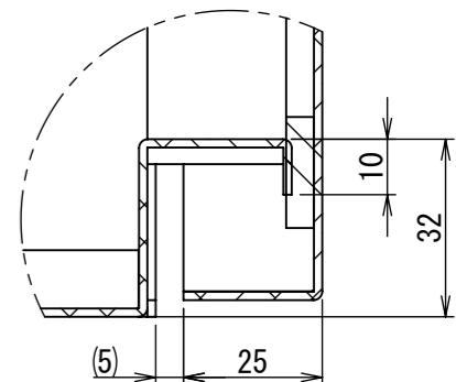
DETAIL C SCALE 2 : 3
